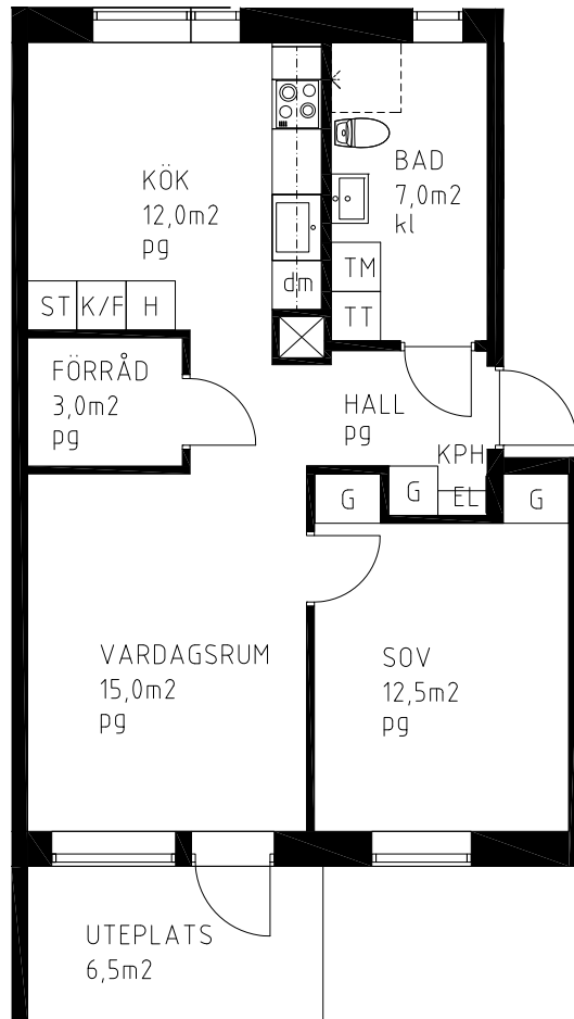
PLAN 1
