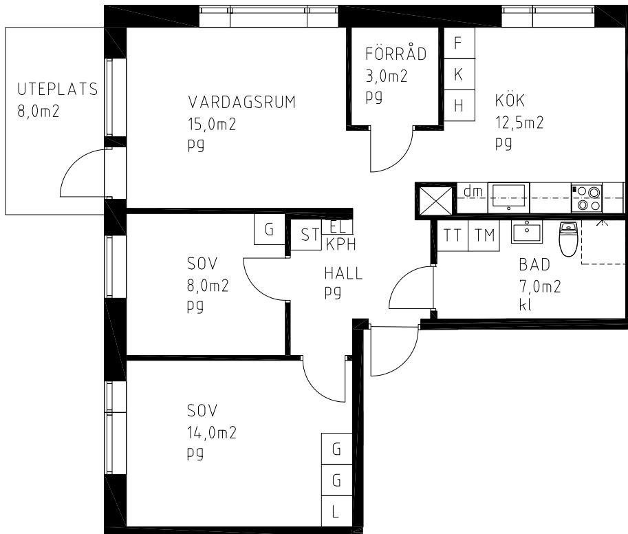
PLAN 4
