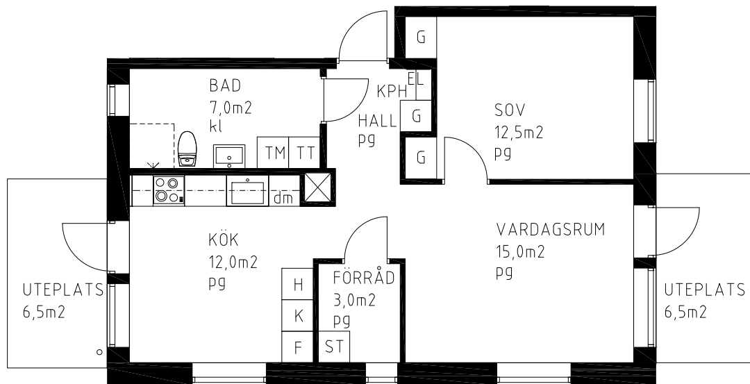
PLAN 1
