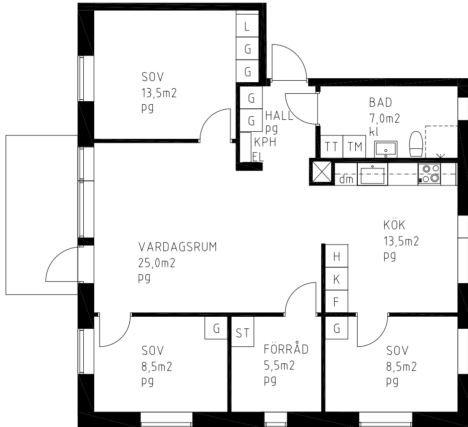
PLAN 2
