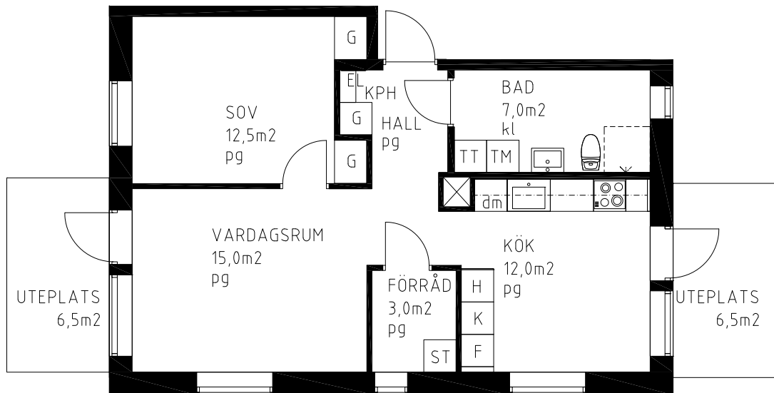
PLAN 1
