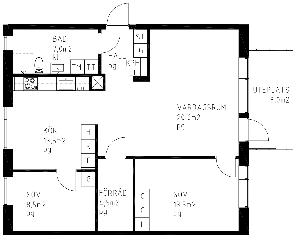
PLAN 2
